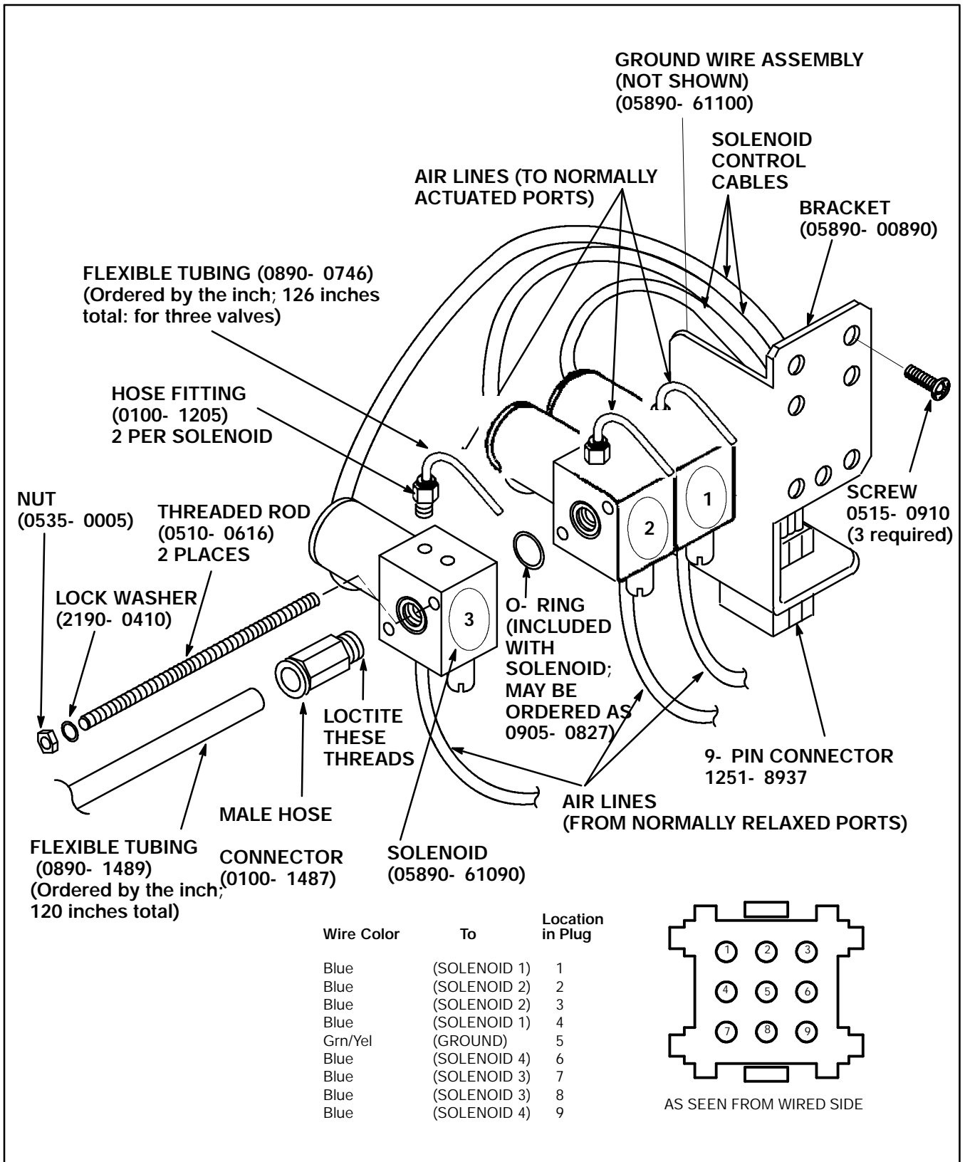
Figure 4. Valve Control Solenoids. (Please see the attached Service Note for Updates.)
